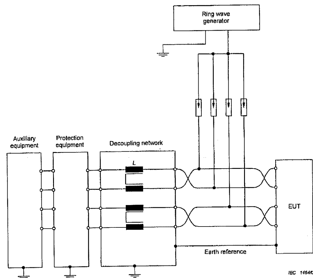
Figure 12 – Example of test setup for unshielded symmetrical interconnection lines (communication lines) – lines-to-ground coupling via arrestors
