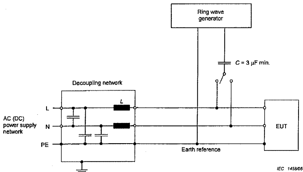
Figure 6 – AC/DC power supply port, single phase, line-to-ground test
